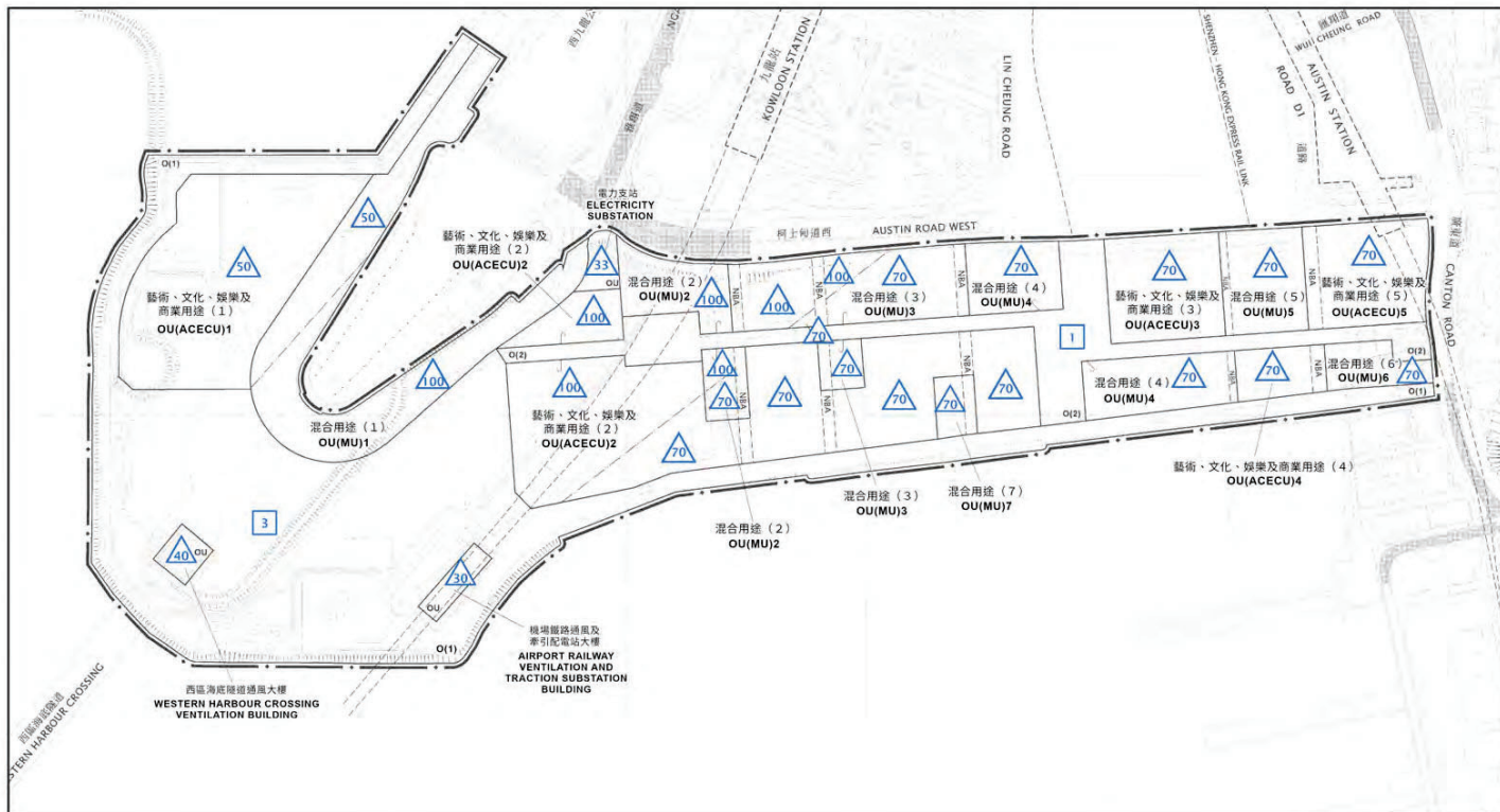
現時在發展圖則上訂明的建築物高度限制 EXISTING BUILDING HEIGHT RESTRICTIONS STIPULATED UNDER DEVELOPMENT PLAN
